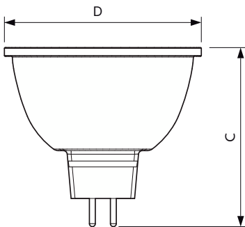
MR16 12V 7-50W 530lm 36D 4000K GU5.3 D
