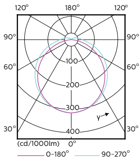
Light Distribution Diagram - LED PLC 8.5W 865 2P G24d-3
