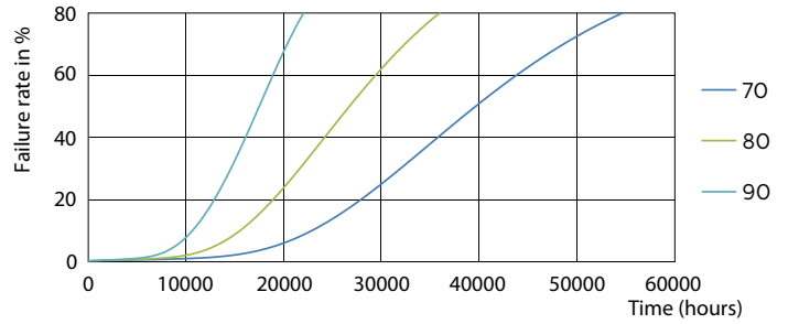
Life Expectancy Diagram - LED PLC 8.5W 865 2P G24d-3
