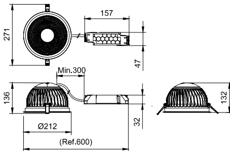
DN591B LED20/830 PSU C D200 WH WB WP GM
